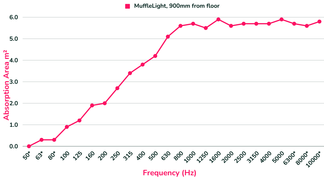
MuffleLight Equivalent Absorption Area per Object
